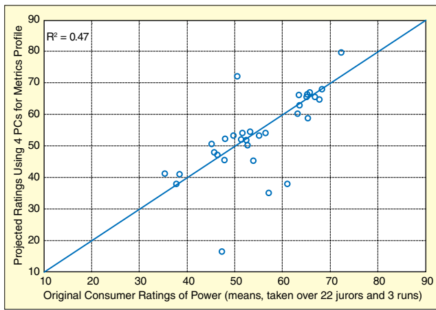
Figure 2. Jury ratings on the attribute “perceived power” (on a normalized scale of 0-100) for the sounds of 32 different versions of a piece of yard maintenance equipment, vs. ratings predicted by multiplying an SQ “metrics profile” derived from these same sounds by a transformation vector.
