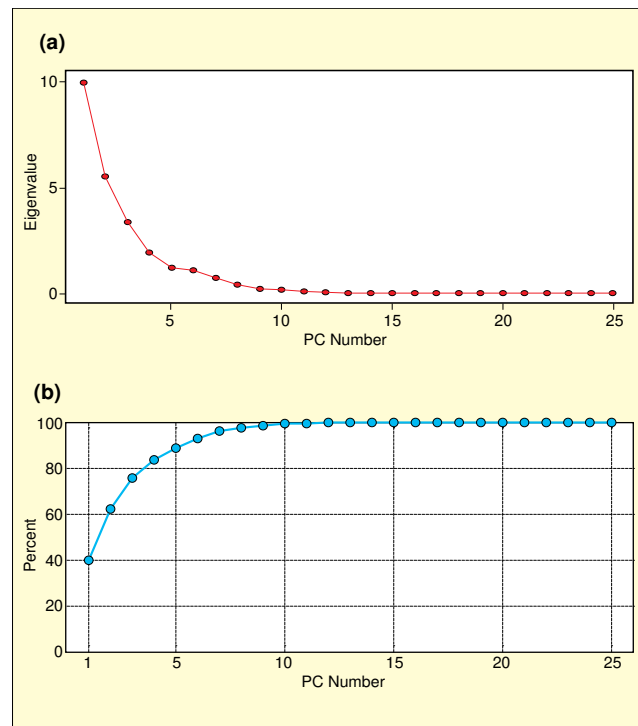
Figure 1. Judging “importance” of the principal components obtained from a set of 25 sound quality metrics calculated for 32 different sounds: (a) “scree” plot of the eigenvalues, (b) cumulative percentage of observed variance represented by the PCs.
